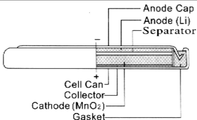
Cutaway View
