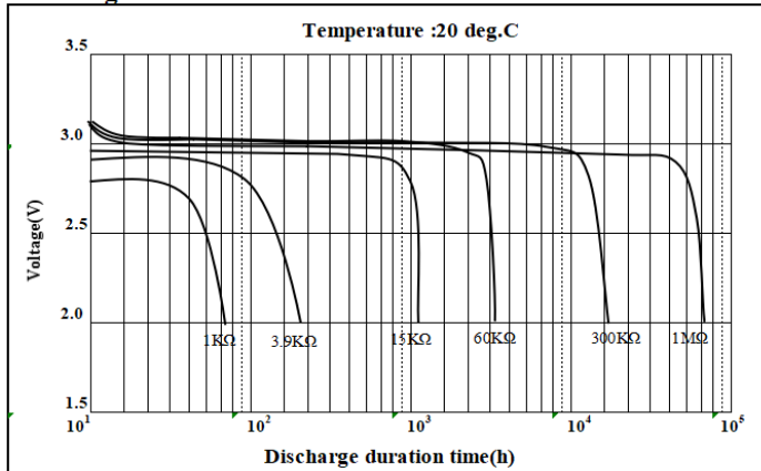
Discharge Characteristics
