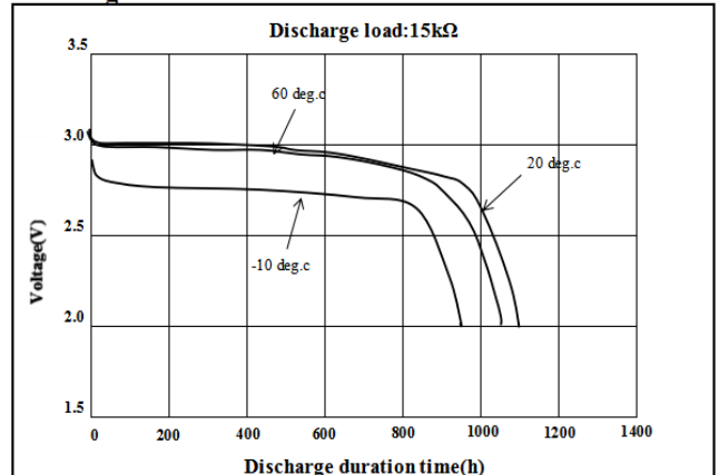
Discharge Characteristics
