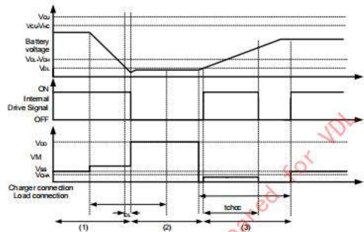
Figure4-3 Abnormal Charger Detection
